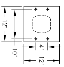
PEDESTAL DETAIL
